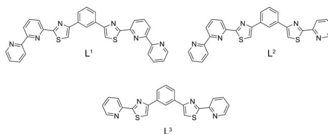
Scheme 1. Multidentate ligands L^1 – L^3 .
